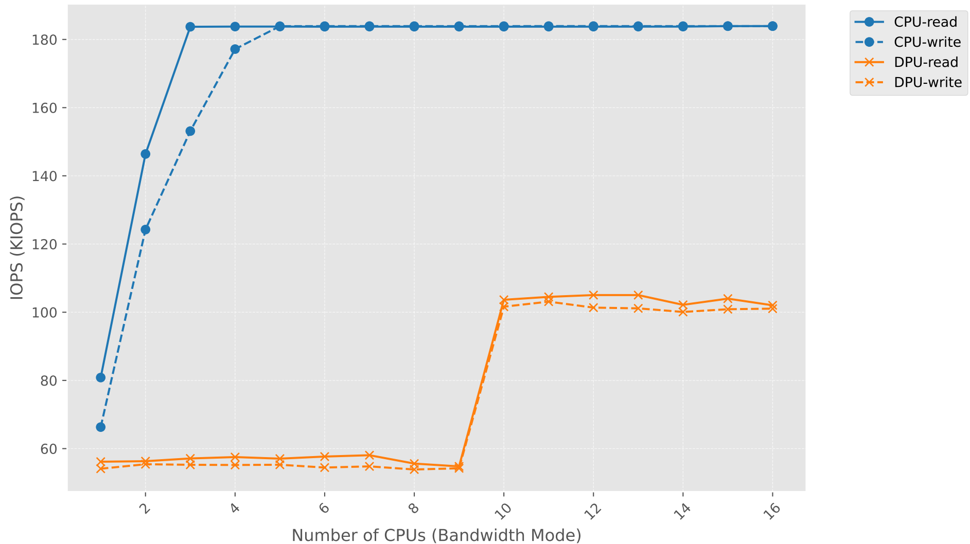
IOPS vs Number of CPUs (Bandwidth Mode)
